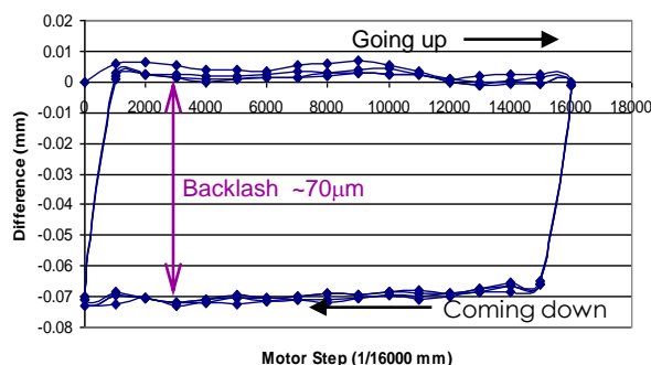
A plot showing the difference between actual position and an ideal straight line over 1mm. Repeated over 3 cycles
